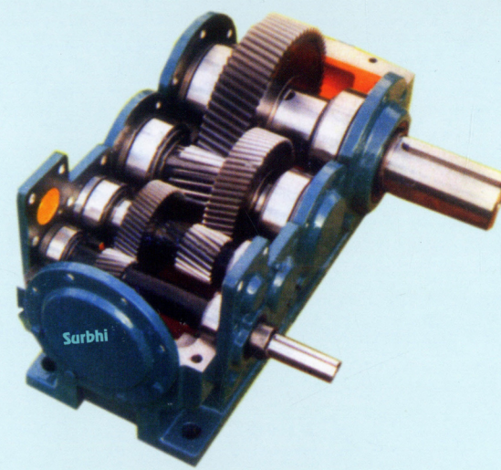
Helical Gear Box
